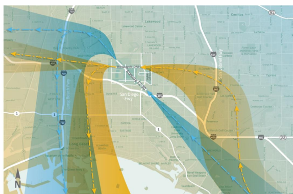
Temporary Runway 12-30 Closure | March 29 - July 18, 2023
